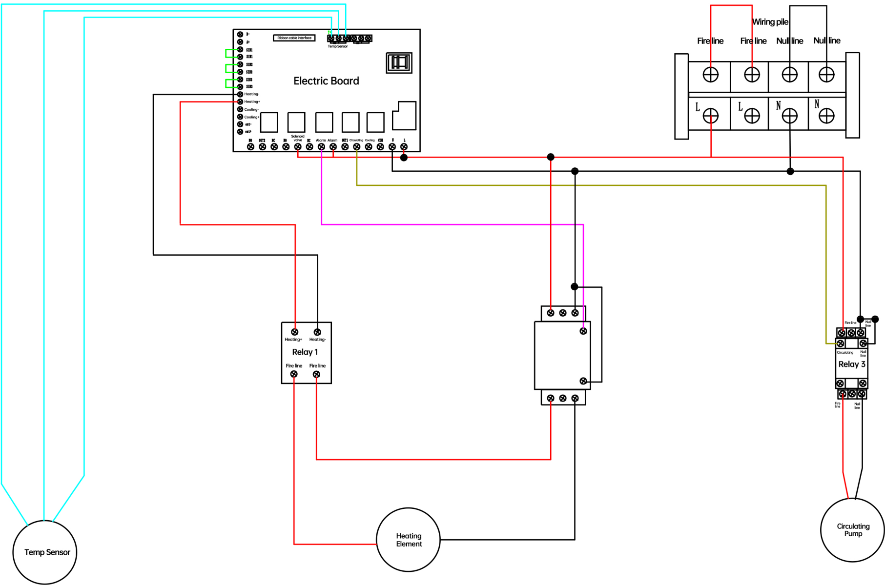
CRH Wiring Diagram
